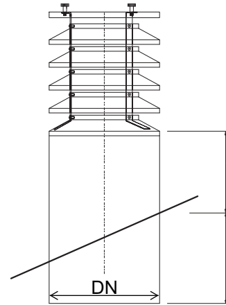
Type CRL-SH-S
