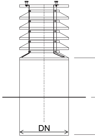
Type CRL-SH-F
