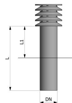
Type CRL-F
