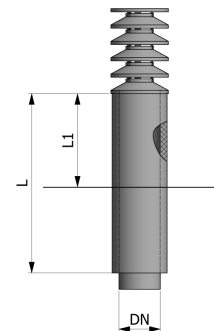
Type CRLD-F
